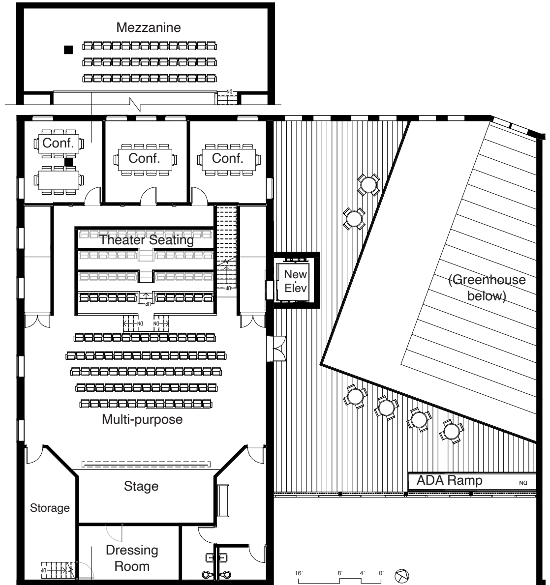
2nd Floor
